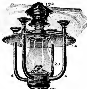
Fig. 3316. CENTER-LAMP. Four-arm Drop.
